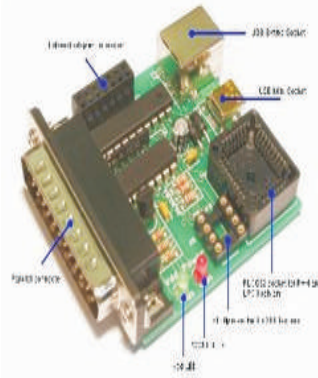
Bios Programmer
